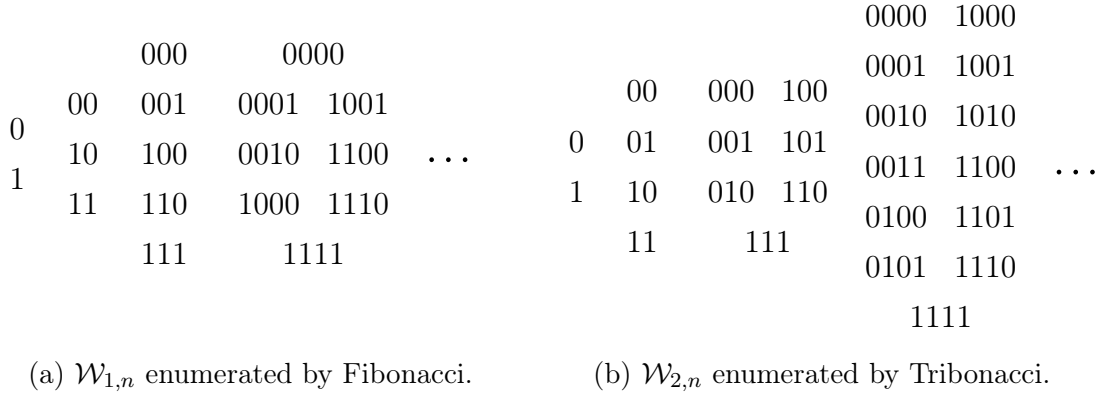
Figure 1: Sets \mathcal{W}_{q,n} for small values of n and q .
